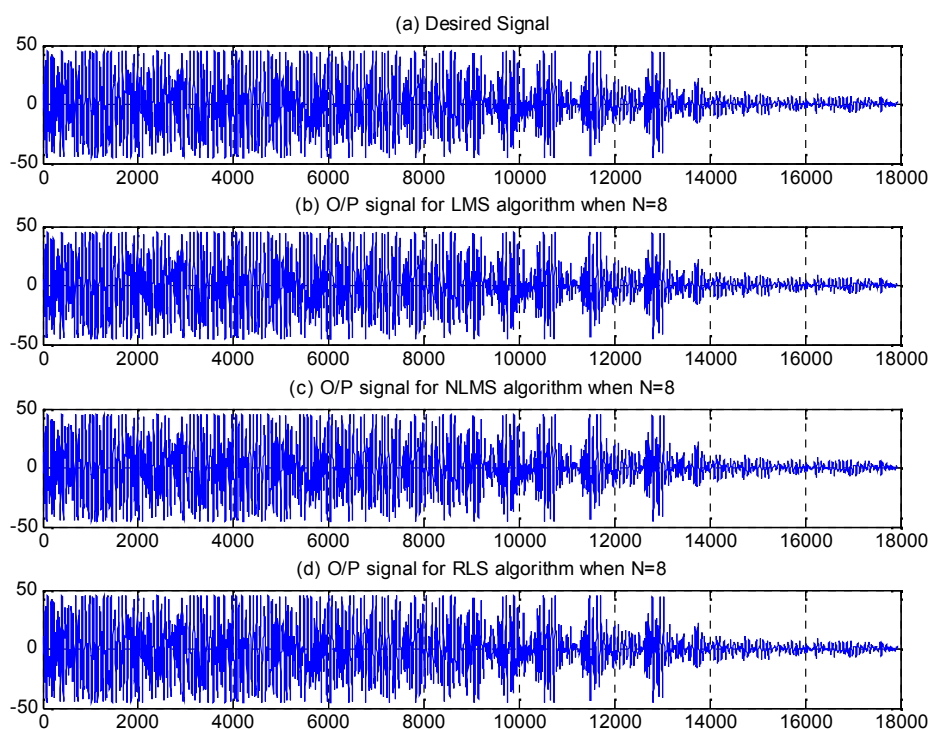
Figure 3:(a) Noisy speech desired signal d(n) ;(b)The simulation of the GAF( LMS) algorithm is carried out with the following specifications: N=8 optimal solution, step size \mu= 0.01 and iterations=18000; (c) NLMS output for same parameters; (d) RLS output filter.
