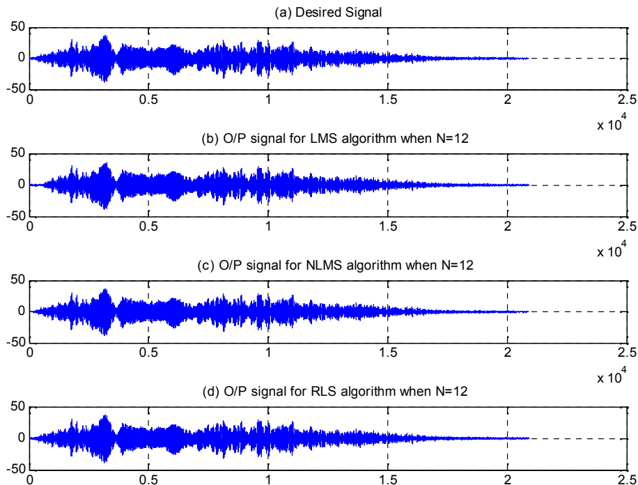
Figure 5:(a) Noisy speech desired signal d(n) ;(b)The simulation of the GAF( LMS) algorithm is carried out with the following specifications: N=12 optimal solution, step size \mu= 0.01 and iterations=250000; (c) NLMS output for same parameters; (d) RLS output filter.
